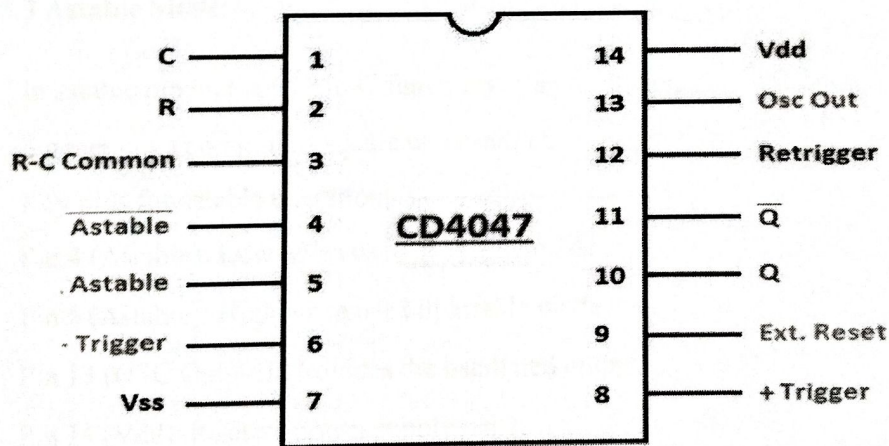
Fig 2.4 IC CD4047 Pinout diagram
