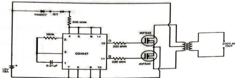
Fig 2.2 Circuit diagram of DC to AC inverter
