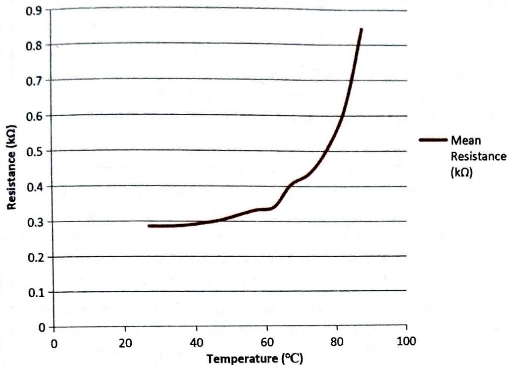
Fig 5.2.2(a) The graph shows an increasing trend of resistance with increasing temperature for carbon film resistors, indicating positive temperature dependence.
