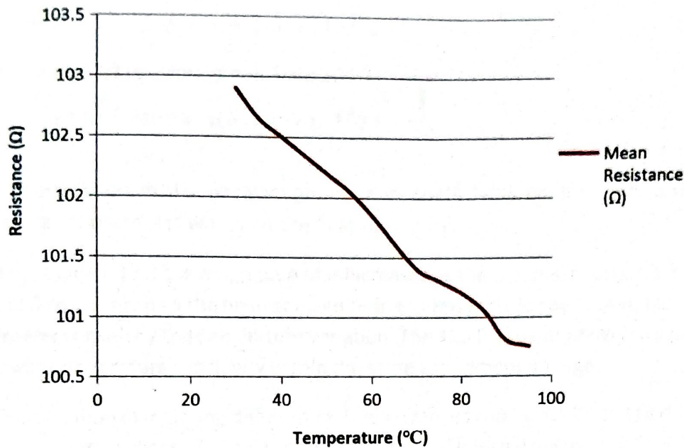
Fig 4.2.2(a) The graph shows a decreasing trend of resistance with increasing temperature for carbon film resistors, indicating negative temperature dependence.
