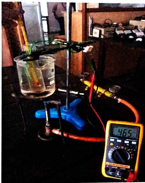
Fig.2.3(a) Experimental setup
