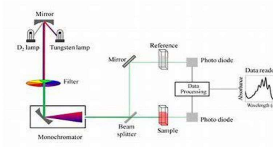
Figure 2.4: UV-vis-NIR spectrophotometer 4
