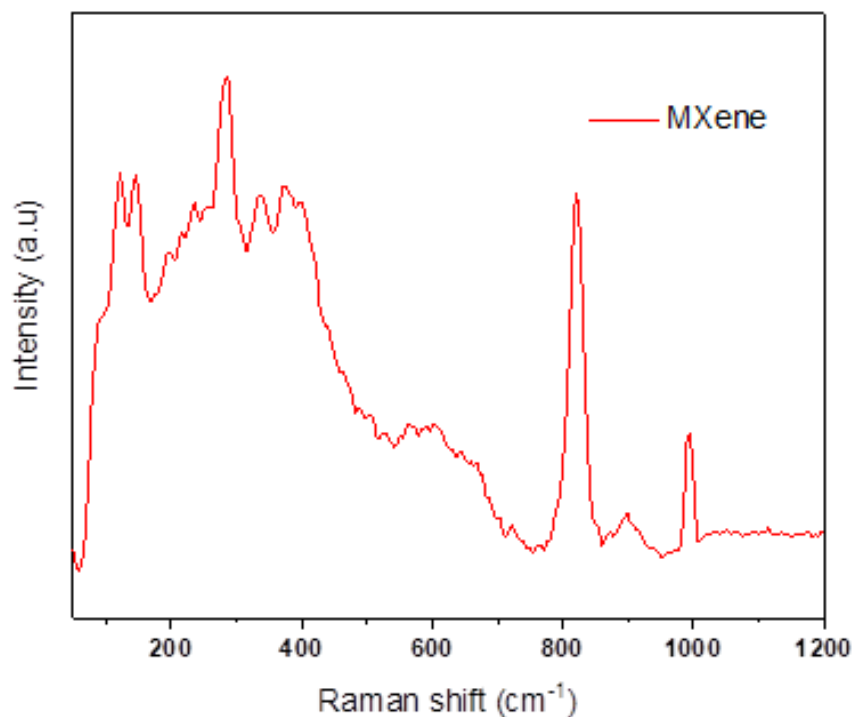
Fig 4.3 Raman spectra of MXene
