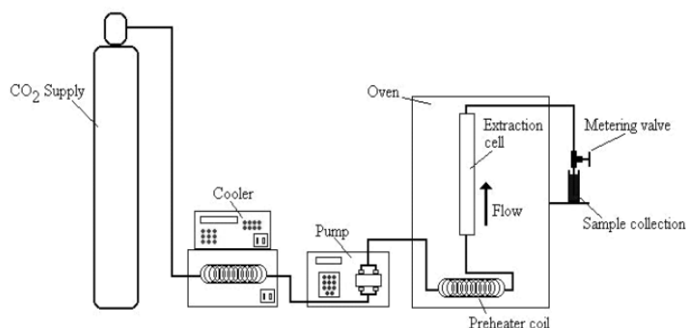
Figure 1.18: Schematic diagram of supercritical fluid extraction apparatus [55]
