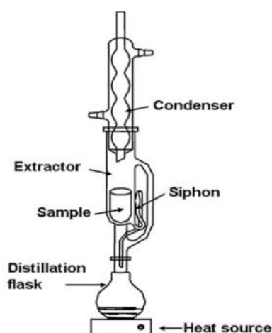
Figure 1.17: Soxhlet extractor [53]
