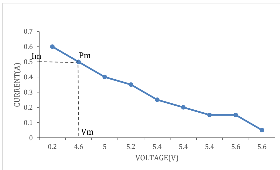
Figure 3.9.1 V-I CHARACTERISTIC CURVE AT 8 DEGREE
