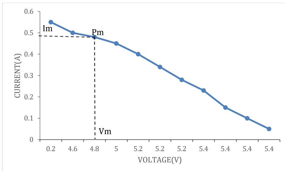
Figure 3.13.1 V-I CHARACTERISTIC CURVE AT 4 DEGREE
