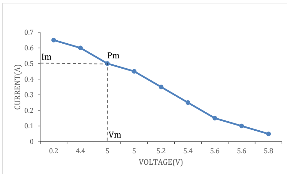
Figure 3.4.1 V-I CHARACTERISTIC CURVE AT 13 DEGREE
