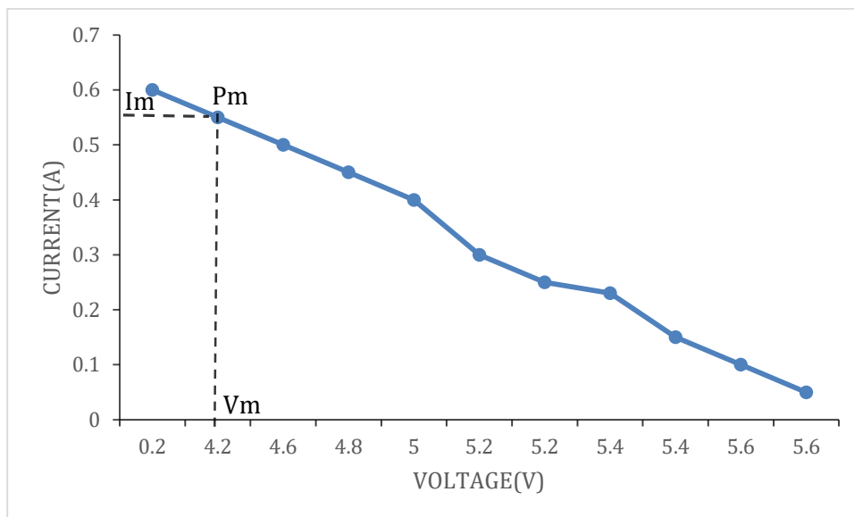
Figure 3.12.1 V-I CHARACTERISTIC CURVE AT 5 DEGREE
