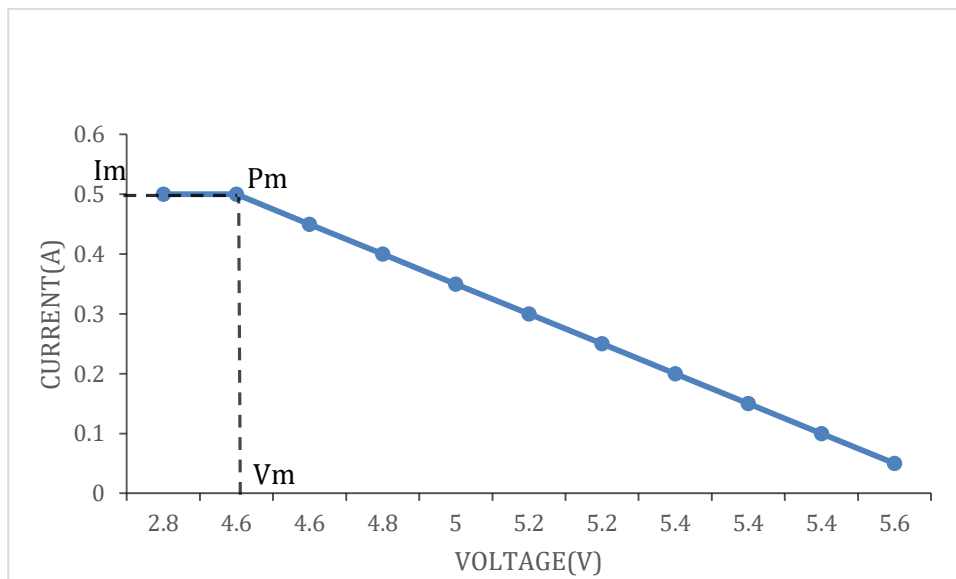
Figure 3.11.1 V-I CHARACTERISTIC CURVE AT 6 DEGREE
