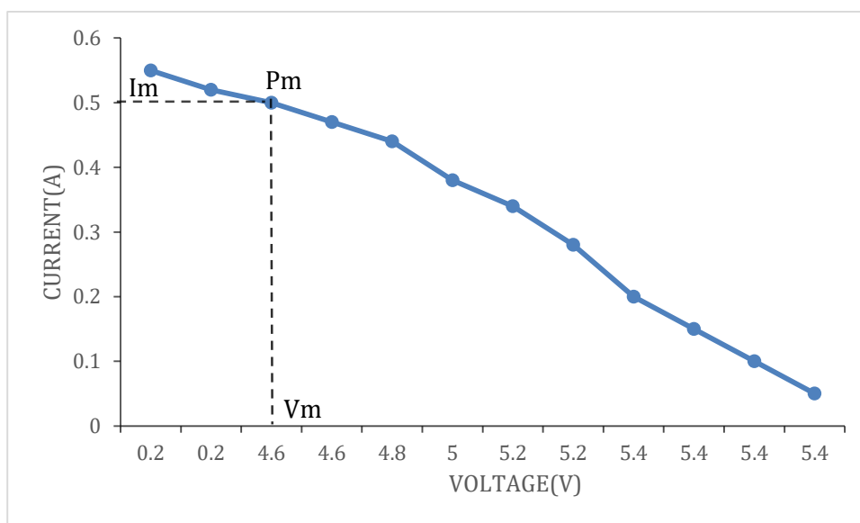
Figure 3.16.1 V-I CHARACTERISTIC CURVE AT 1 DEGREE
