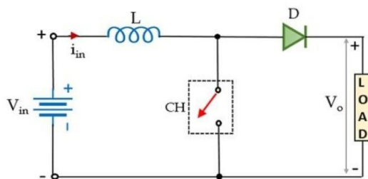
Elementary Circuit of Boost Converter
