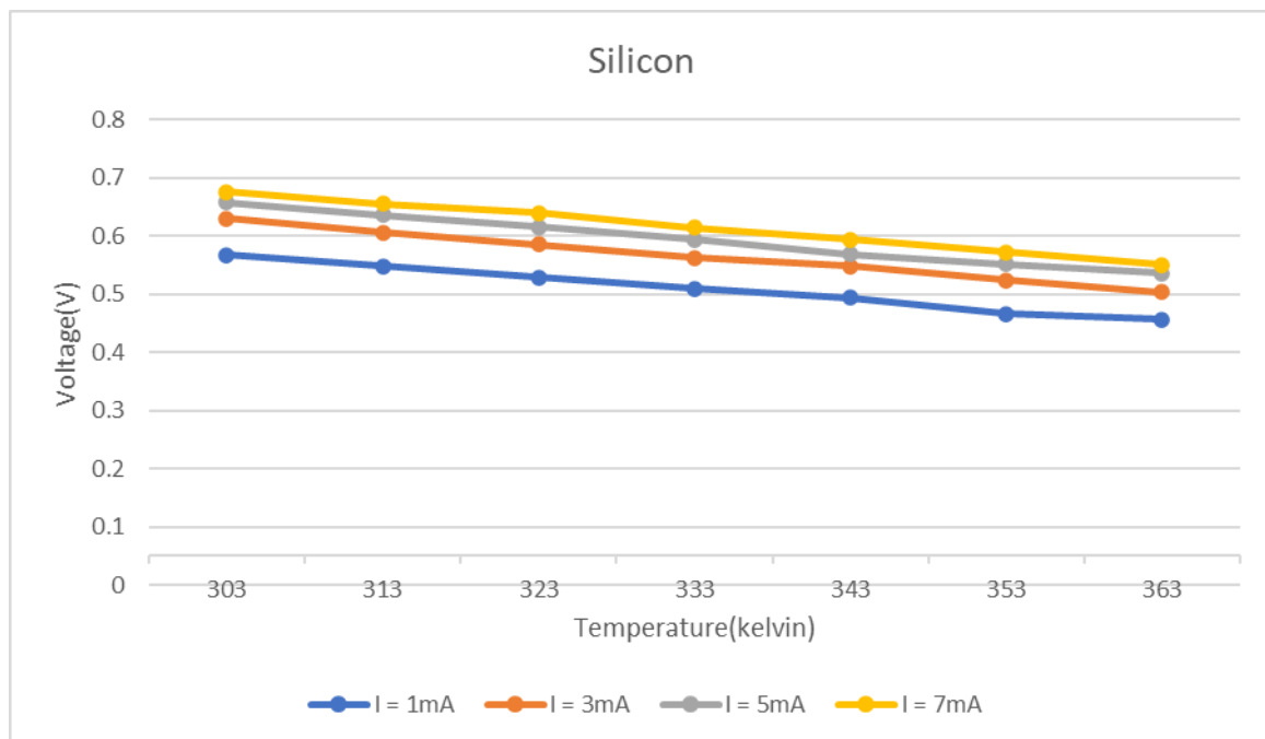
Fig 3.7 Temperature vs Voltage graph of Silicon diode
