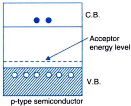
Fig 2.9 Acceptor level of p-type semiconductor
